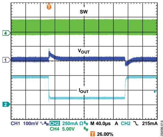
Figure 17. Response to Load Transient, 150 mA to 500 mA, V_{OUT} = 1.8 V, PWM Mode
